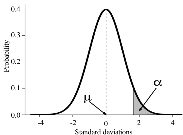
Figure 1. Example of a normal probability density function. \mu represents the mean value and the dark area represents the \alpha value.
